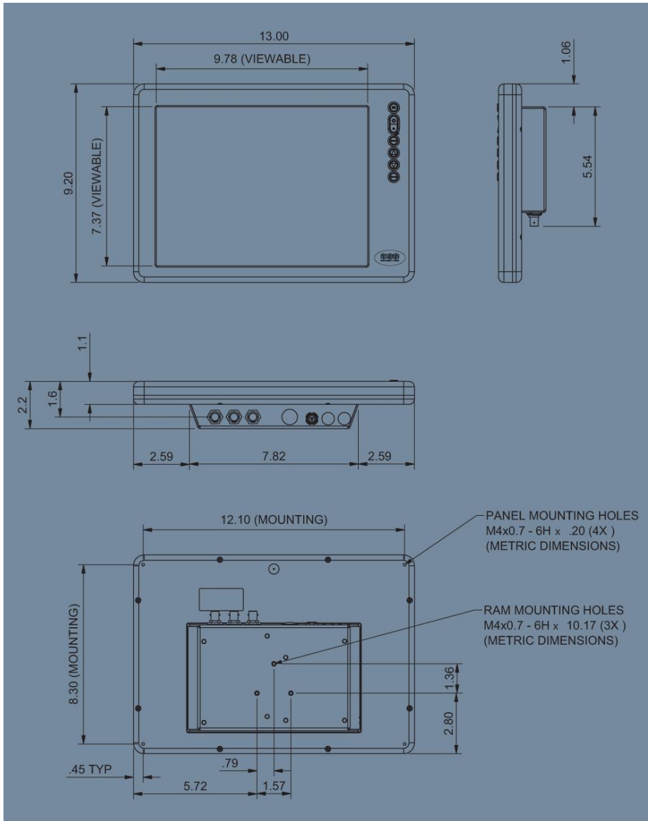
Pictured TOP: Standard DOD Series with Power and BNC (3) Inputs.
